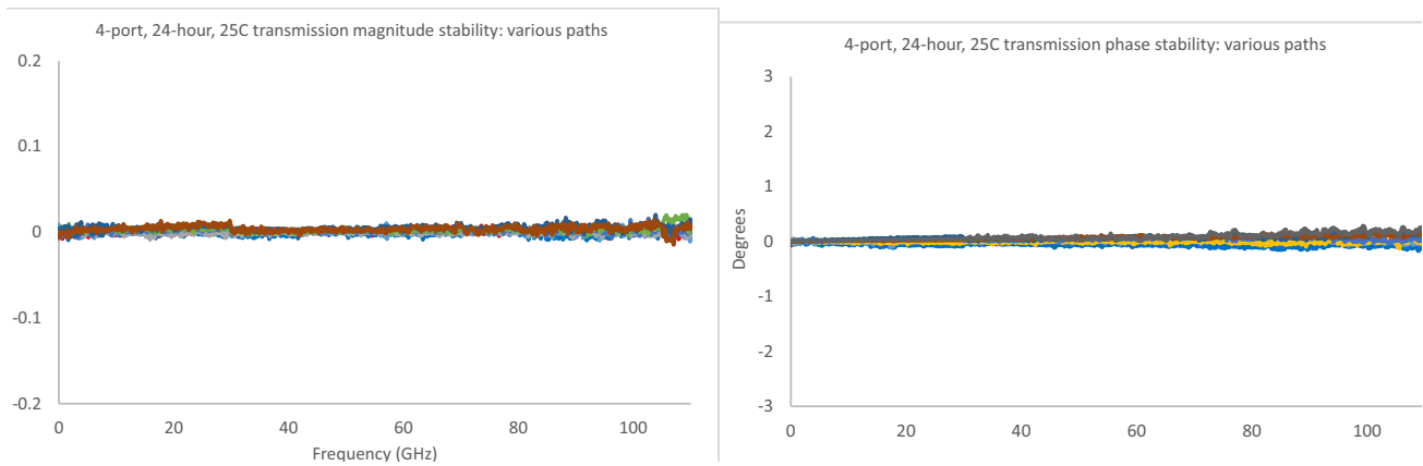
ME7838E4 4-port typical broadband transmission stability over 24 hours with temperature held constant (25 °C). Measurements of thru lines on a sampling of the possible two-port paths are represented.
