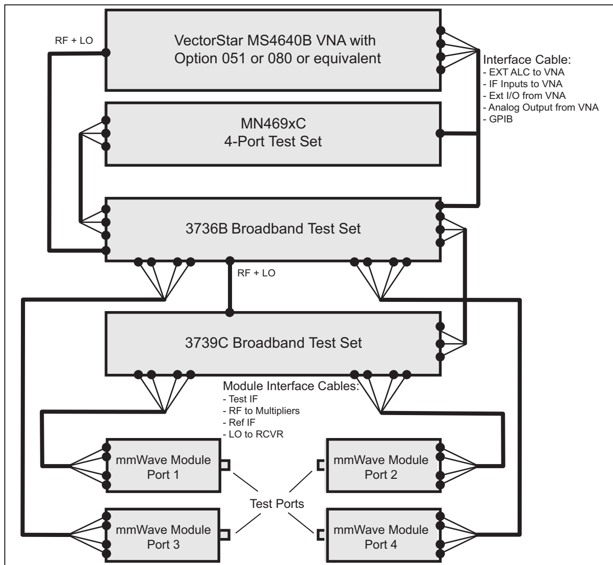
ME7838E4 4-Port Broadband Millimeter-Wave Configuration Block Diagram
