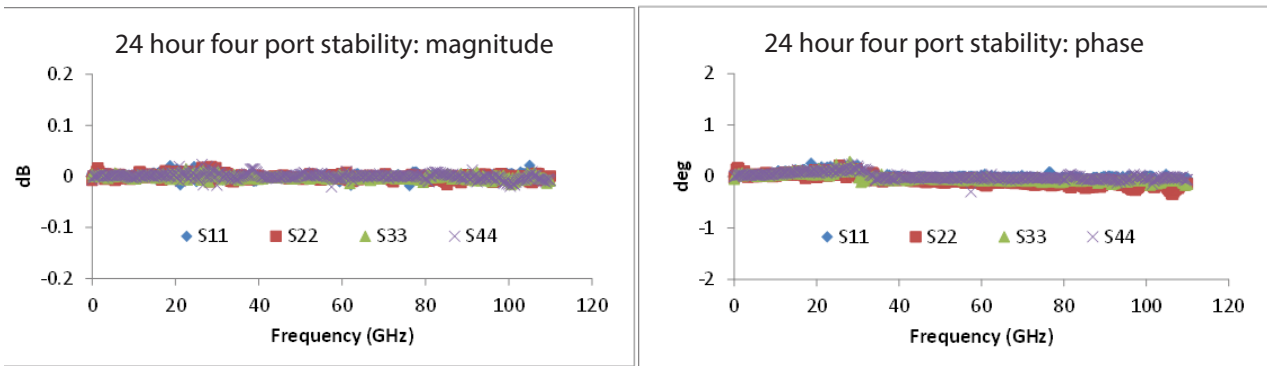
ME7838E4 4-port typical Broadband Reflection Magnitude and Phase Stability with temperature held constant (25 °C).
