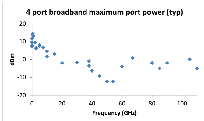
ME7838E4 4-Port Broadband Typical Maximum Port Power. Units with Option 31 will typically have higher maximum power below 54 GHz.
