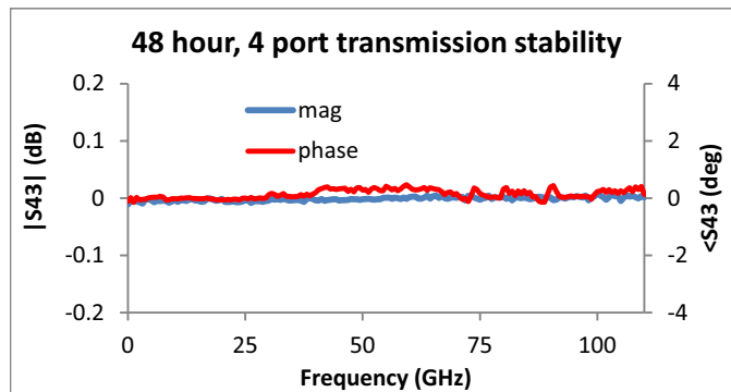
ME7838E4 4-Port Typical Transmission Stability over 48 hours and 6 °C Temperature swing.
