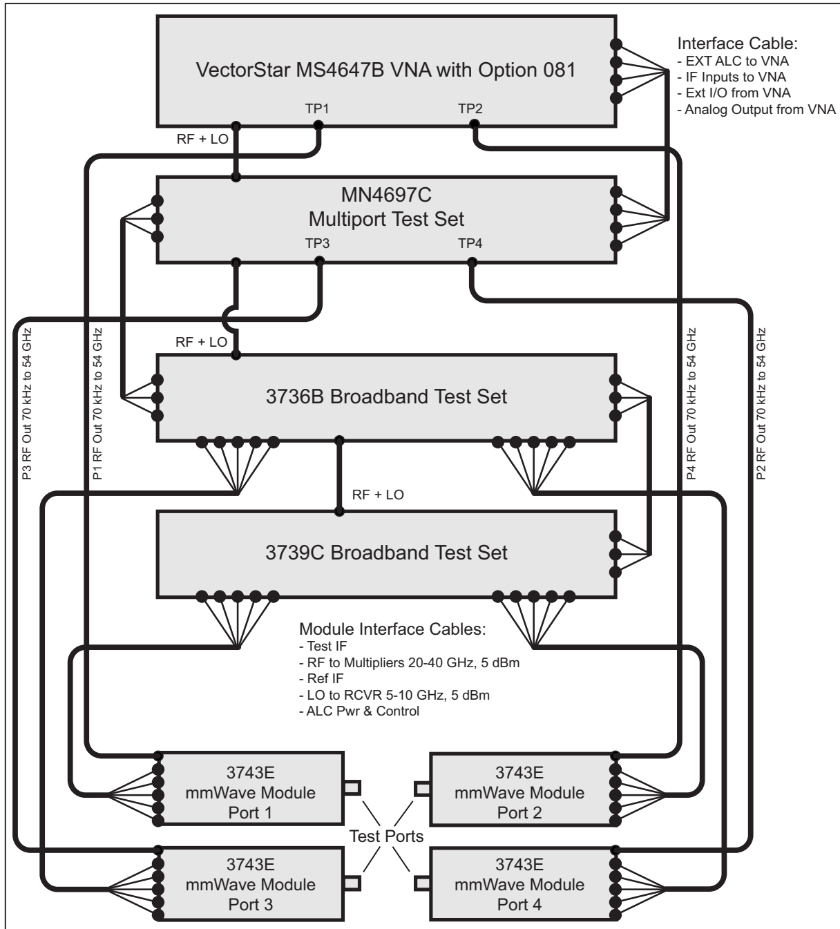
ME7838E4 4-Port Broadband (70 kHz to 110 GHz) Configuration Block Diagram
